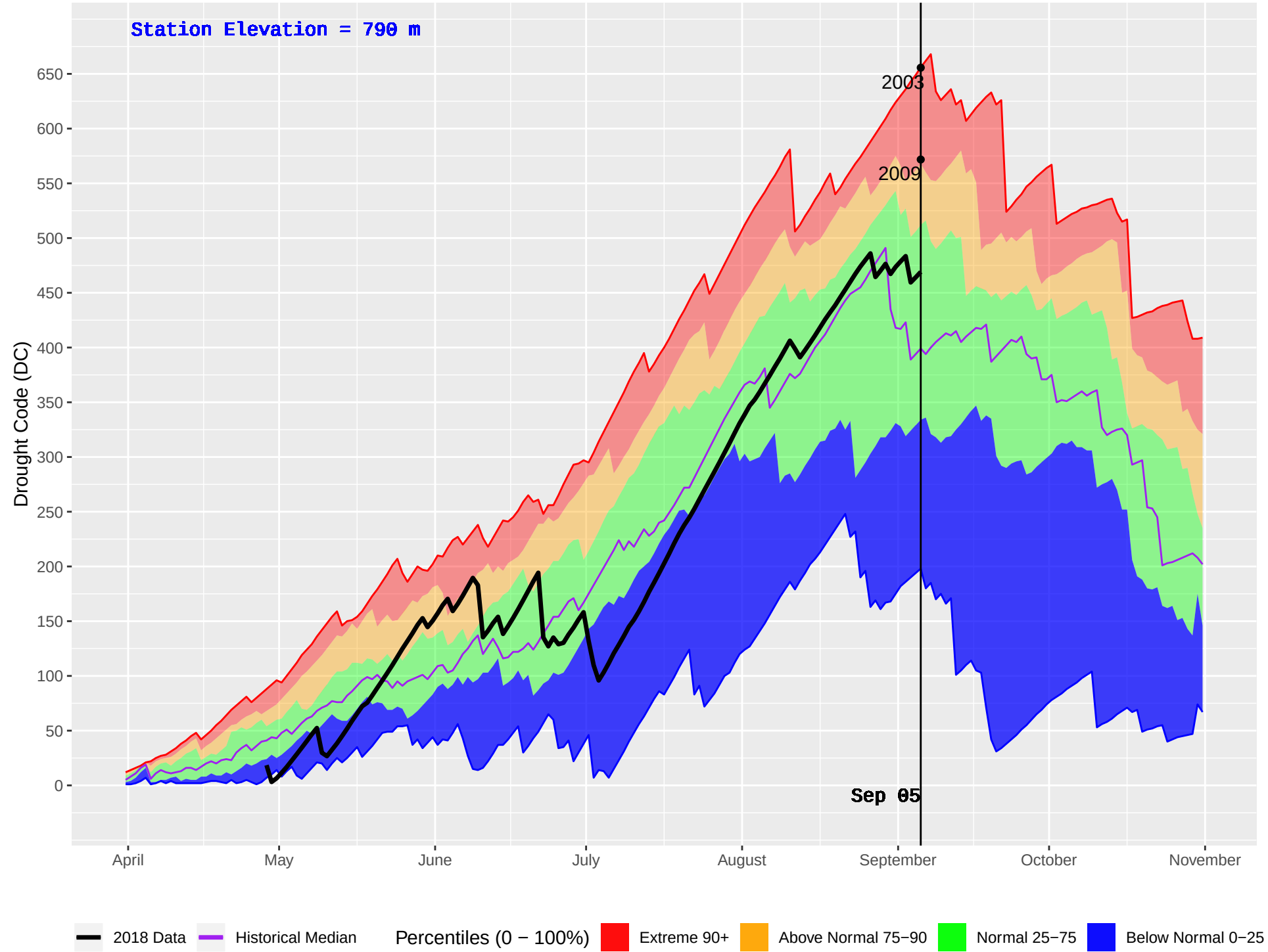
FALLS CREEK (383) : Historical (2002–2016) and Current (2018) Daily Drought Code (DC)
