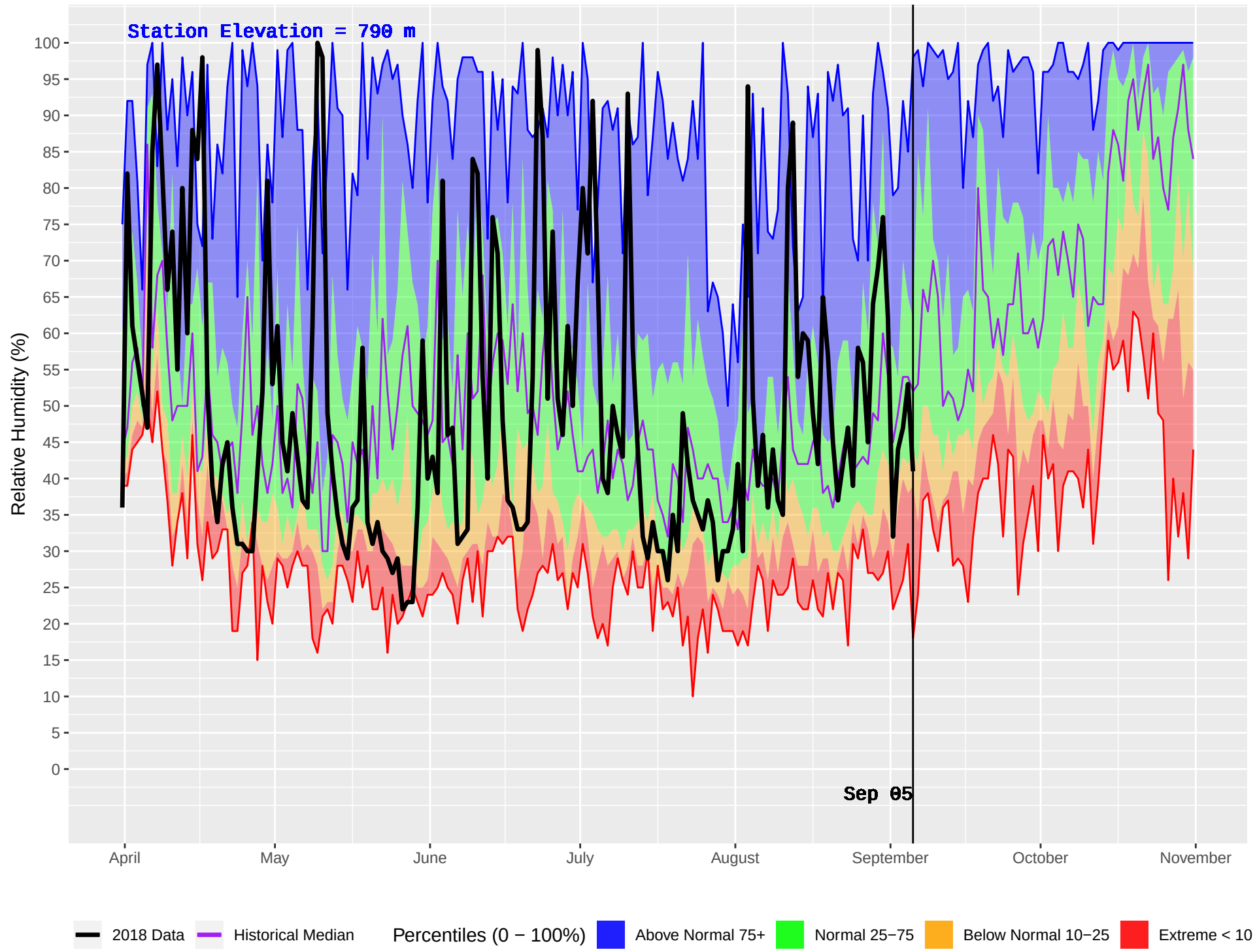
FALLS CREEK (383) : Historical (2002–2016) and Current (2018) Daily Relative Humidity
