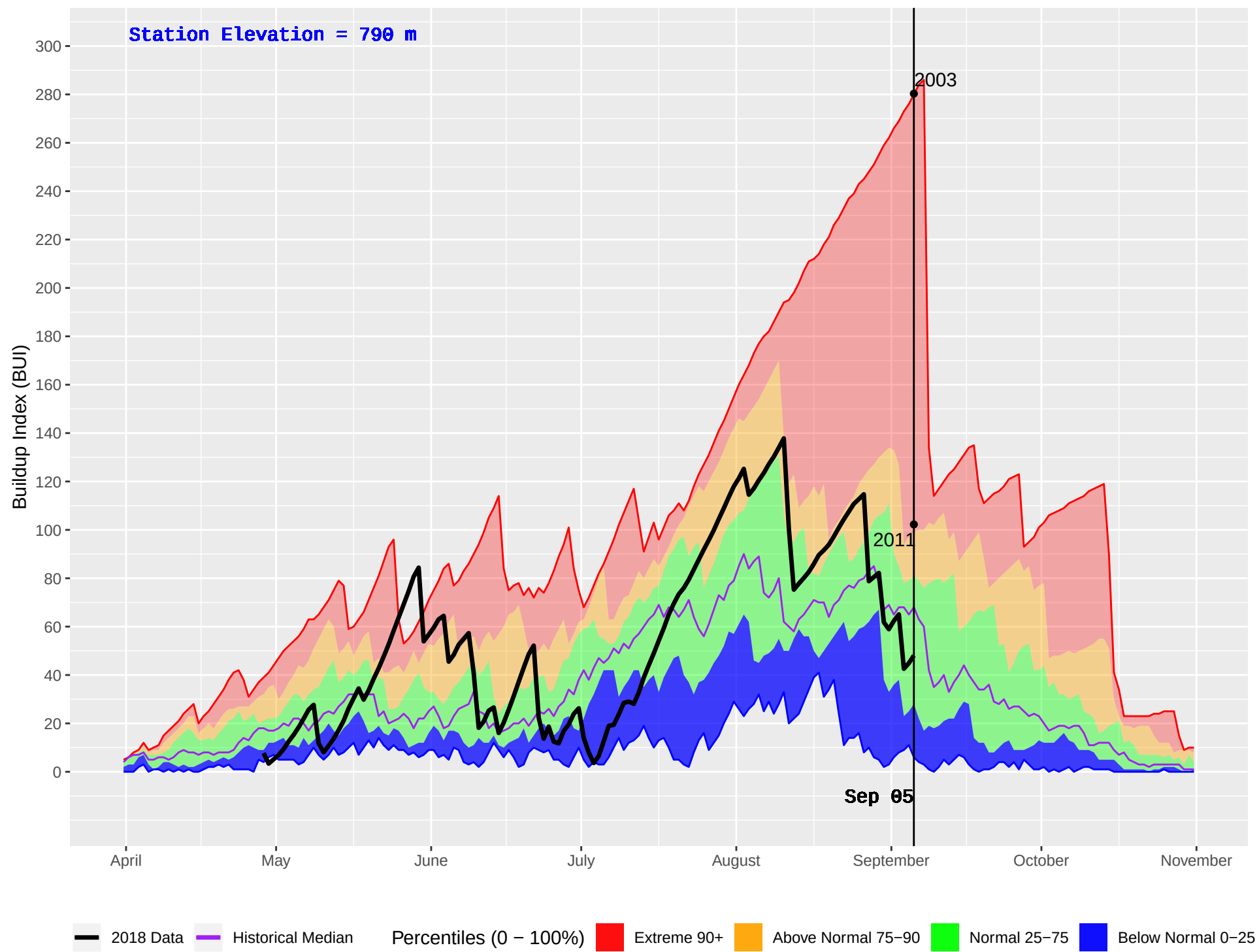
FALLS CREEK (383) : Historical (2002–2016) and Current (2018) Daily Buildup Index (BUI)
