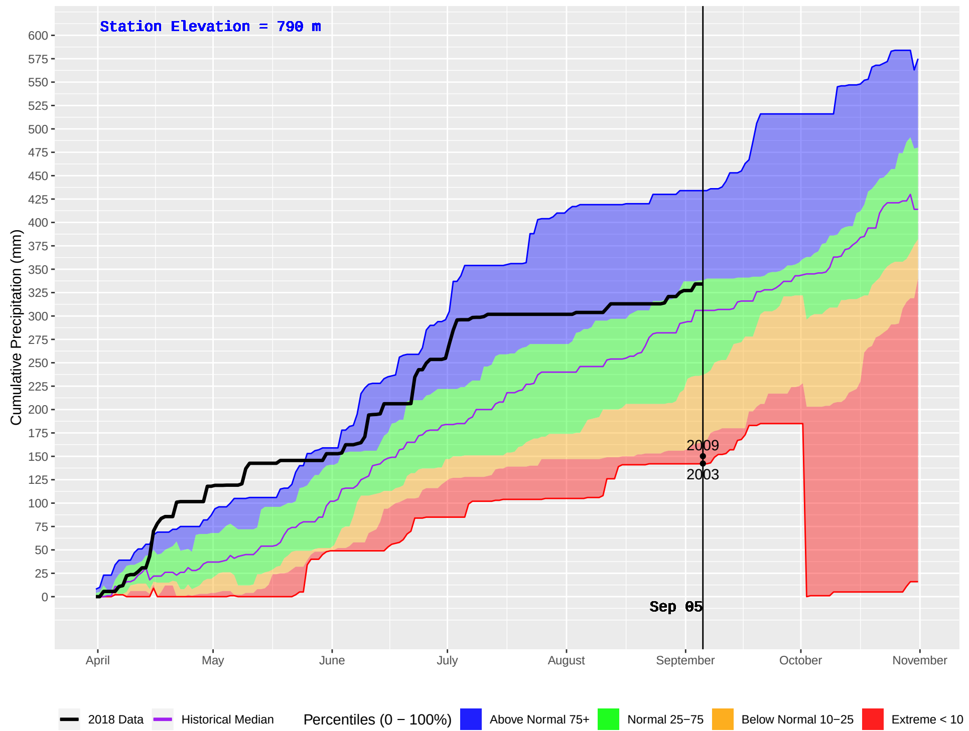
FALLS CREEK (383) : Historical (2002–2016) and Current (2018) Daily Cumulative Precipitation
