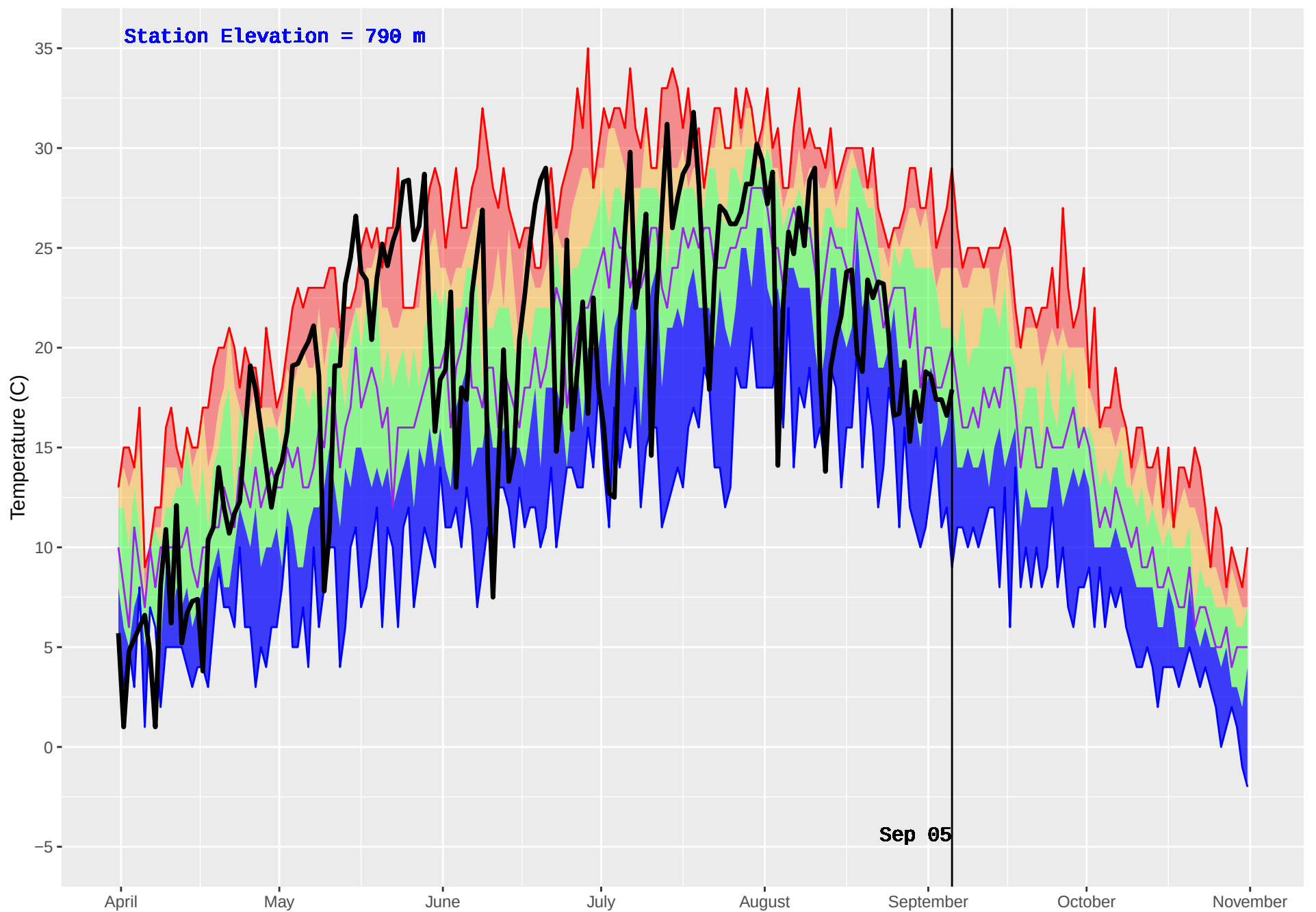
FALLS CREEK (383) : Historical (2002–2016) and Current (2018) Daily Temperature
