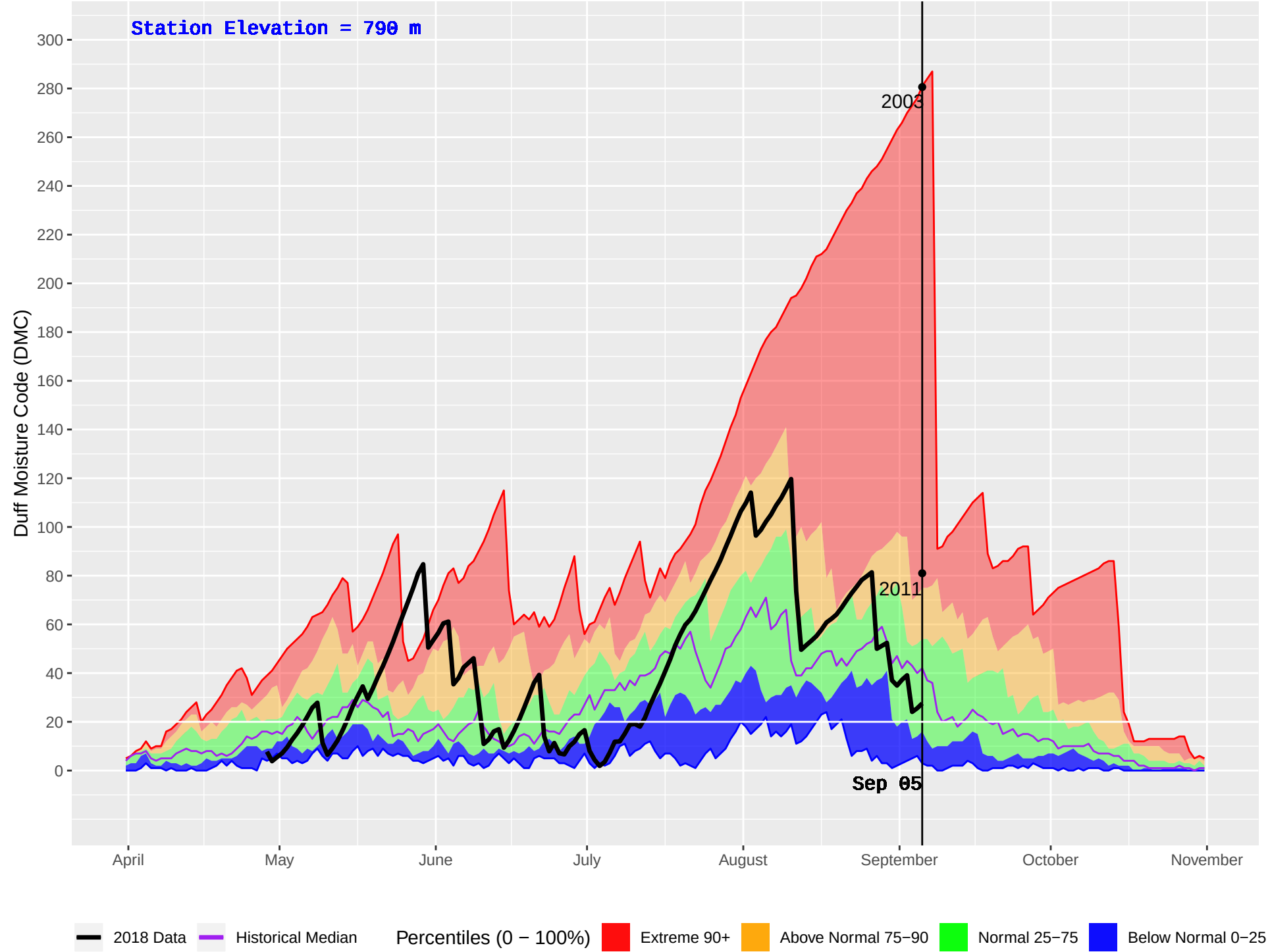
FALLS CREEK (383) : Historical (2002–2016) and Current (2018) Daily Duff Moisture Code (DMC)
