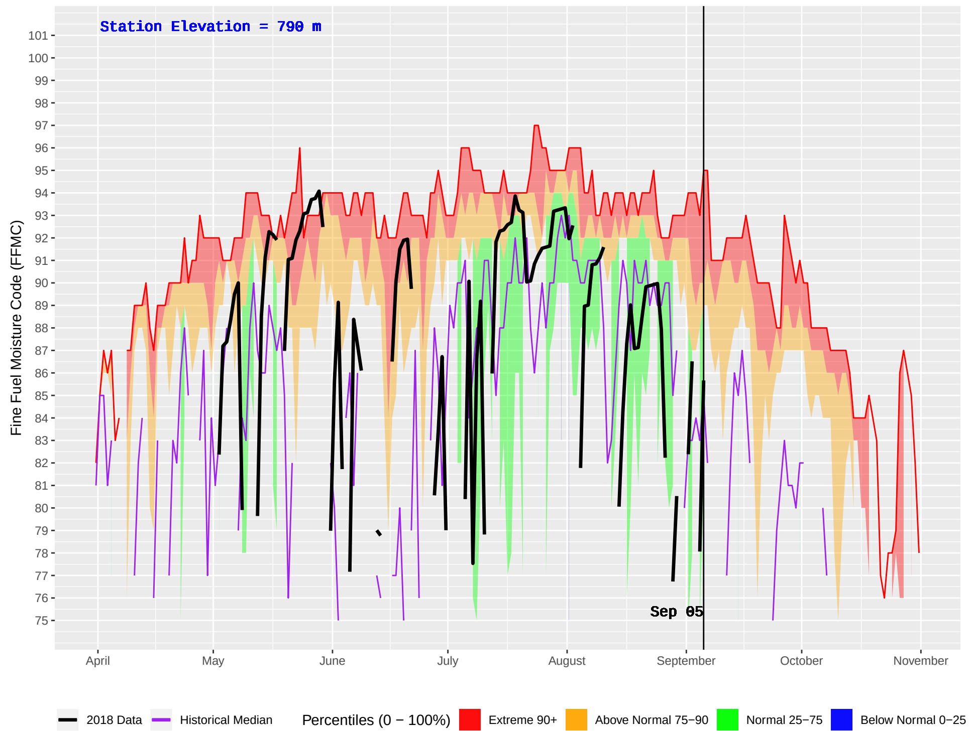
FALLS CREEK (383) : Historical (2002–2016) and Current (2018) Daily Fine Fuel Moisture Code (FFMC)
